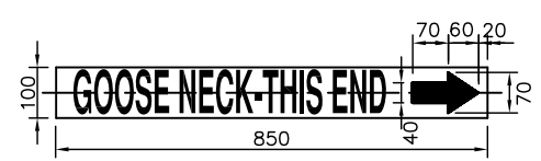
DETAIL 16 1:16
