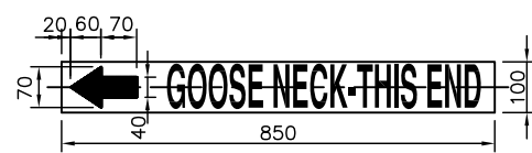
DETAIL 15 1:16
