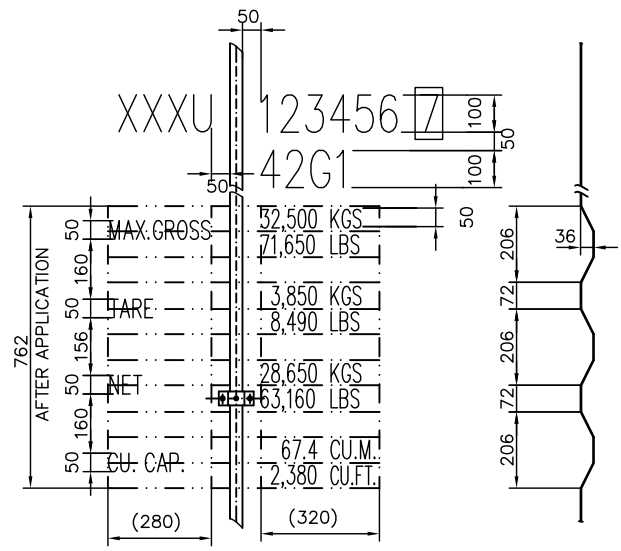
DETAIL 4; 5; 6 1:20
